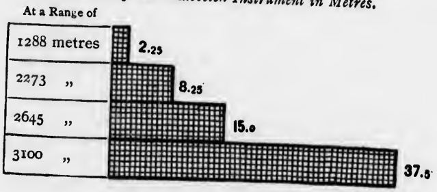
Deviation of the Paskevitch Instrument in Metres.
